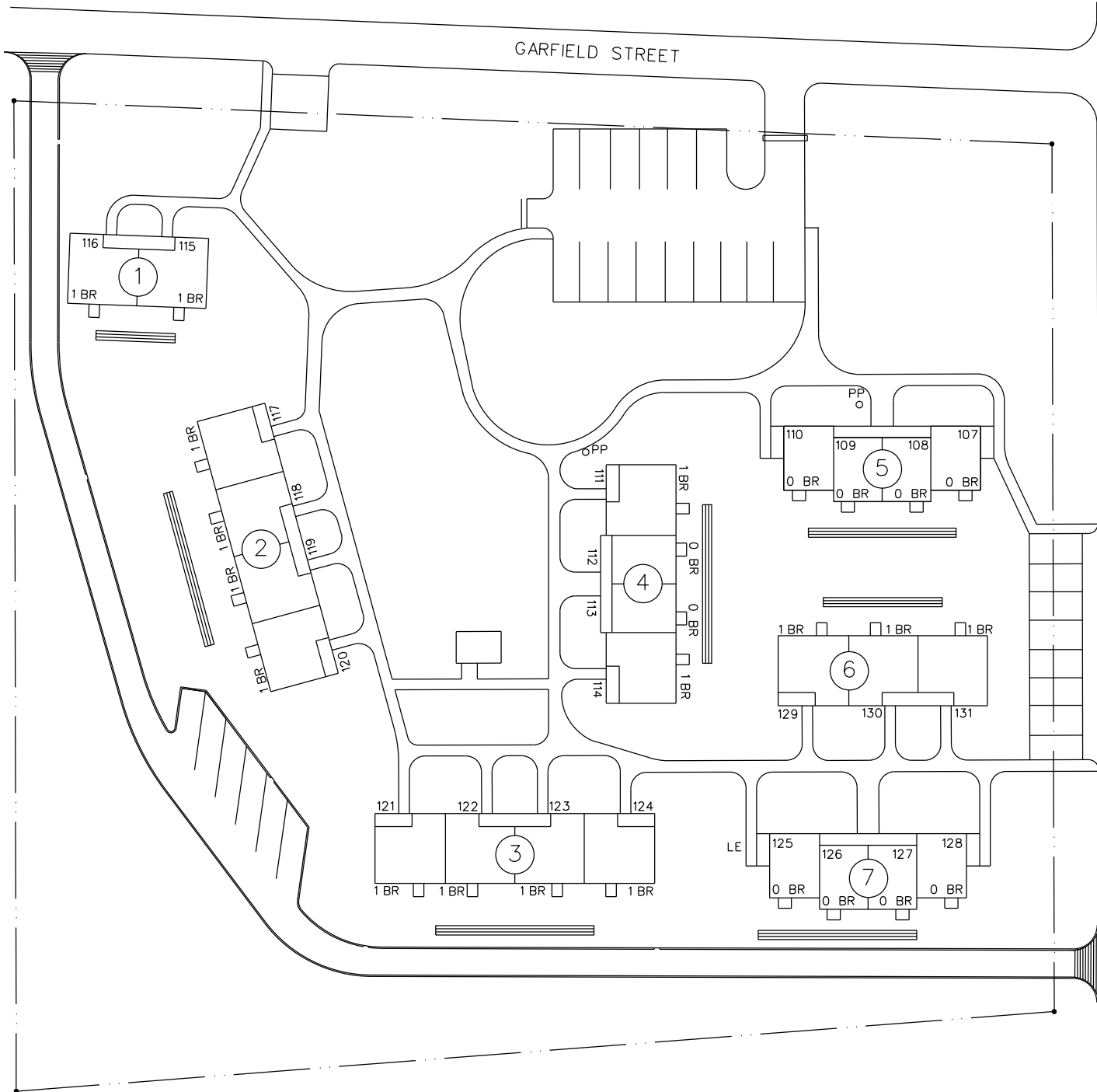
SITE PLAN TN75001-1 SCALE: 1" = 40'-0"
